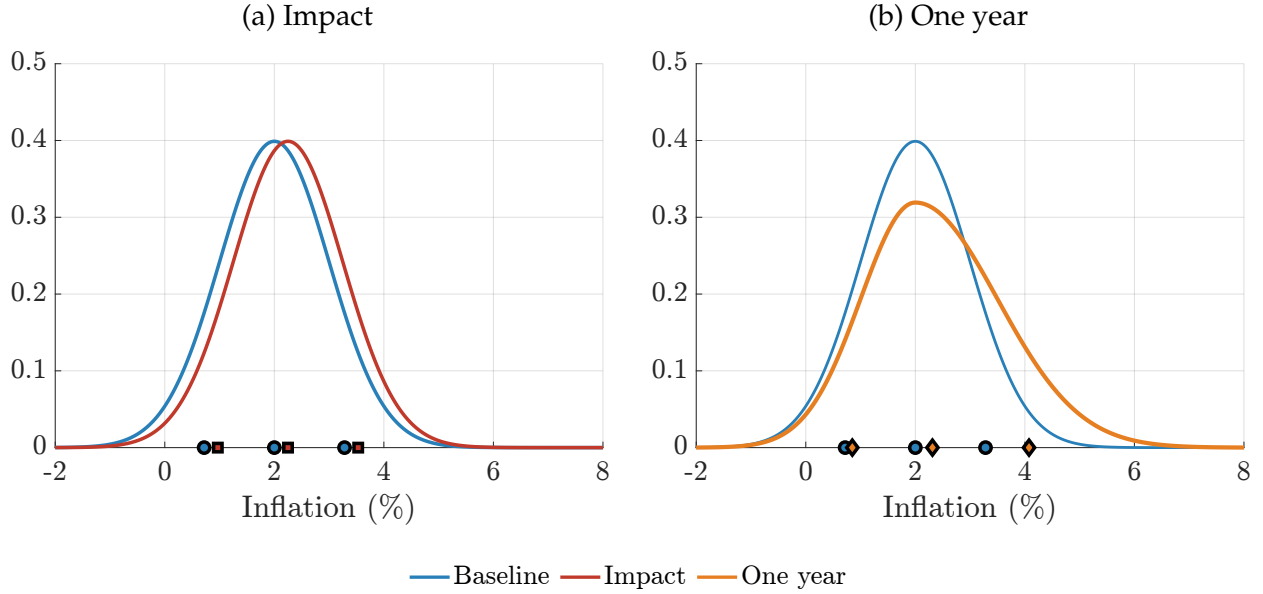
Figure 2: Conditional distributions
